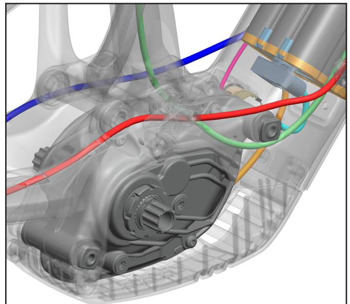
Top View of System Wiring
