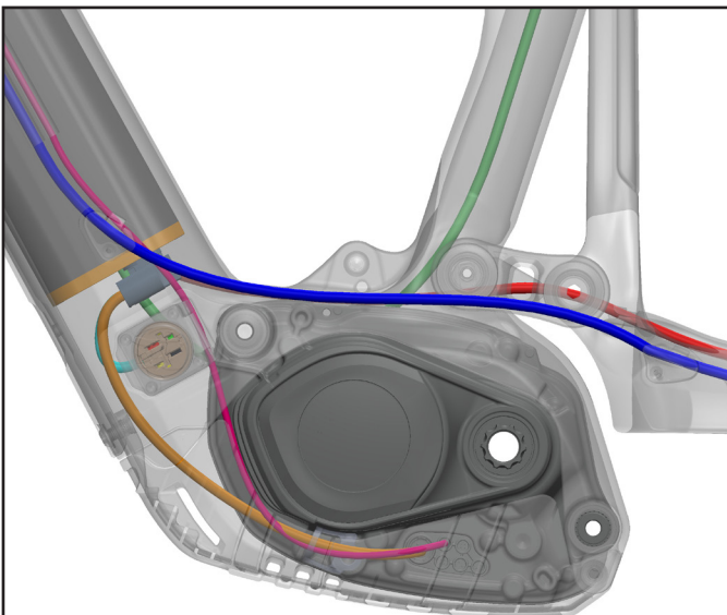
Non-Drive Side View
